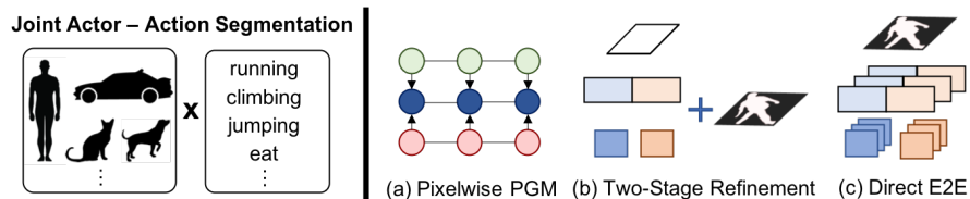
Fig. 1: We tackle the problem of joint actor-action semantic segmentation in videos, which requires simultaneous pixelwise recognition of different actor and action classes. Prior work have proposed (a) pixelwise probabilistic graphical model (PGM) approaches [28, 27] and (b) two-stage refinement approaches [11]. (c) In this work, we propose a new direct end-to-end architecture that combines video action recognition and actor segmentation in a single unified model.
