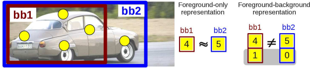
Fig. 4. Bounding boxes bb_1 and bb_2 have a similar foreground-only feature representation, but they are very different under the foreground-background representation. Here, the numbers denote the count of object-related descriptors. For bb_1 , parts of object that leaked into the background will be greatly discounted by the background model.
